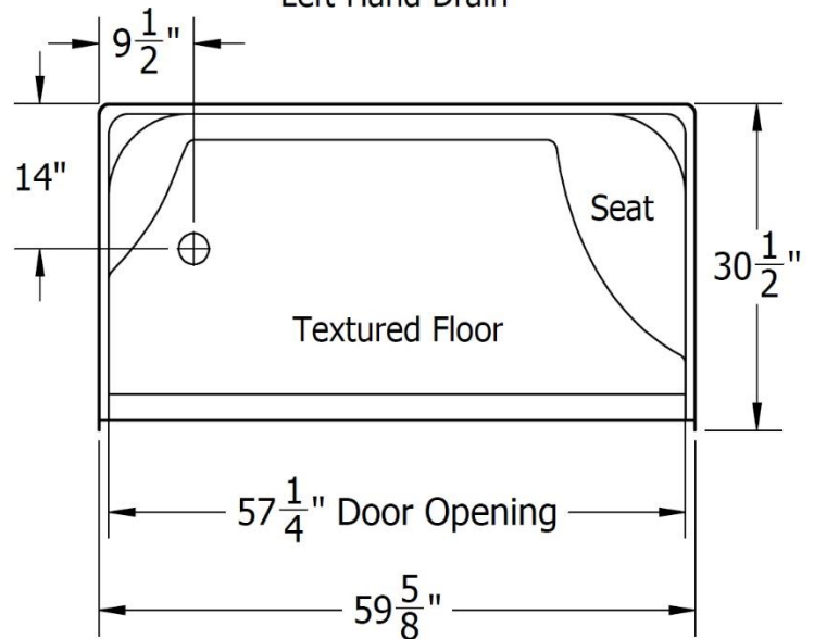
Top View Left Hand Drain
